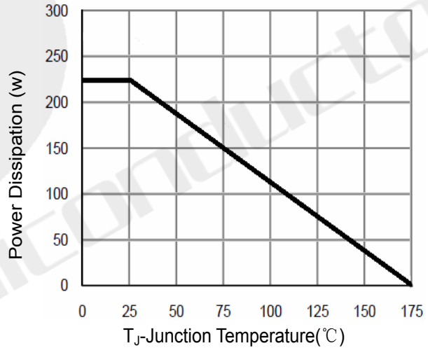
Figure 10 Power De-rating
