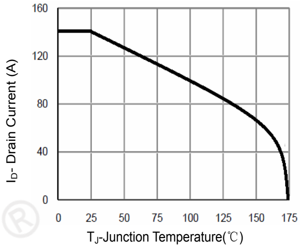
Figure 9 Current De-rating
